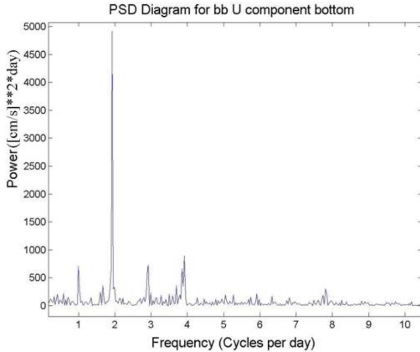
Figure 17. Power spectrum diagram (PSD) for bb u component at the bottom.
